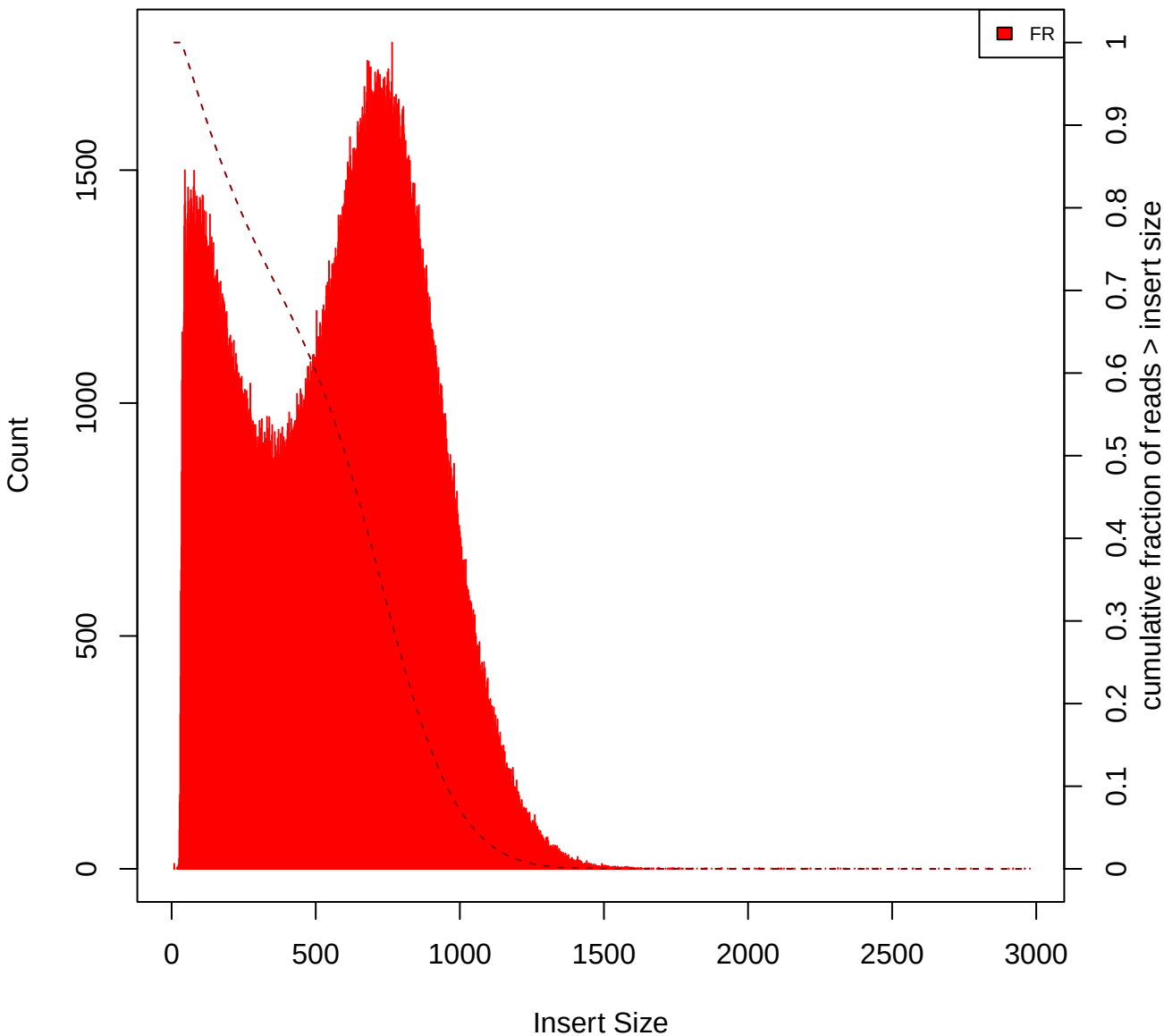
Insert Size Histogram for All_Reads in file SRR2584863_sorted_dedup_reads.bam
