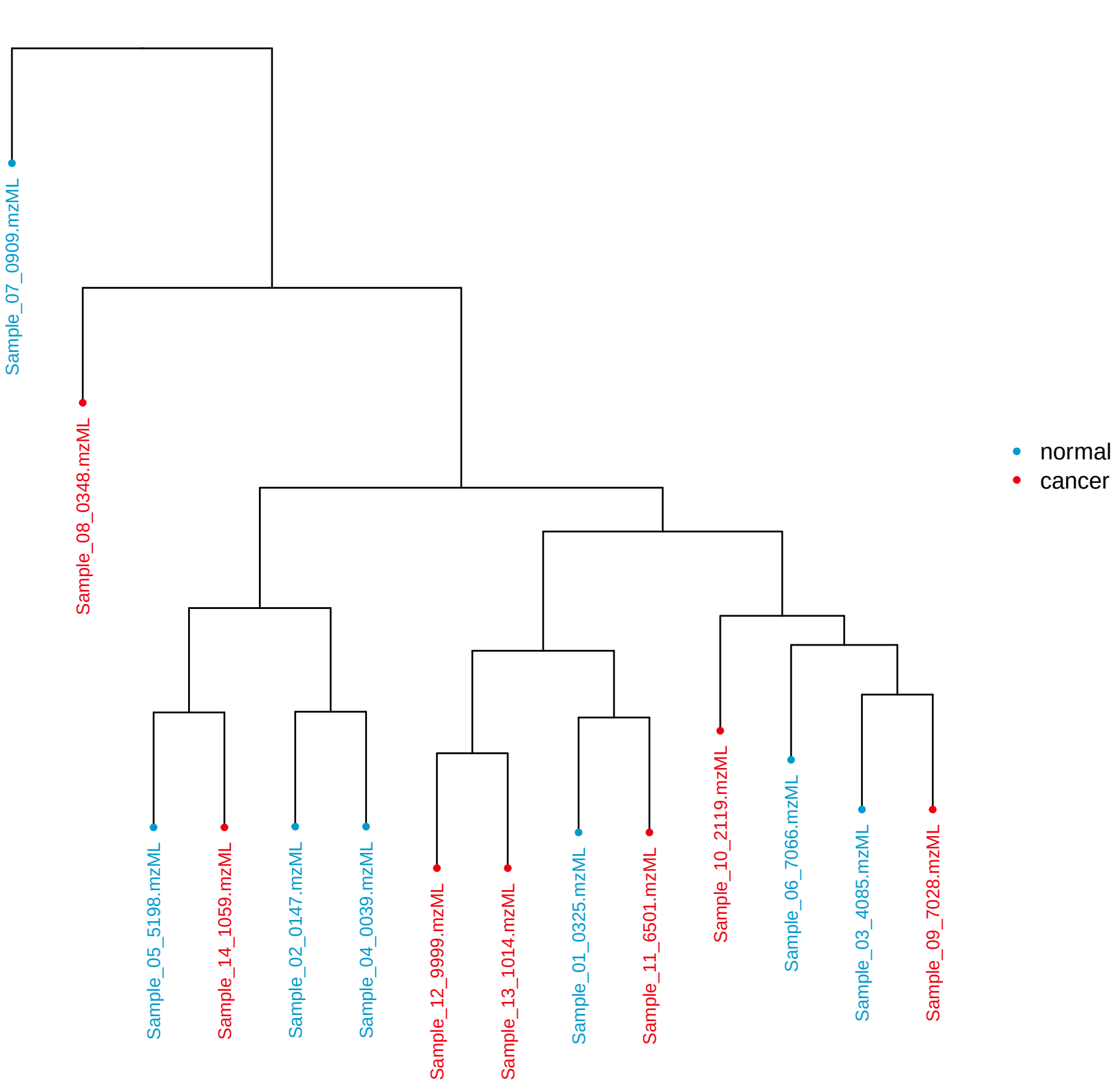
Cluster method: complete Distance metric: euclidean Colored by: group
