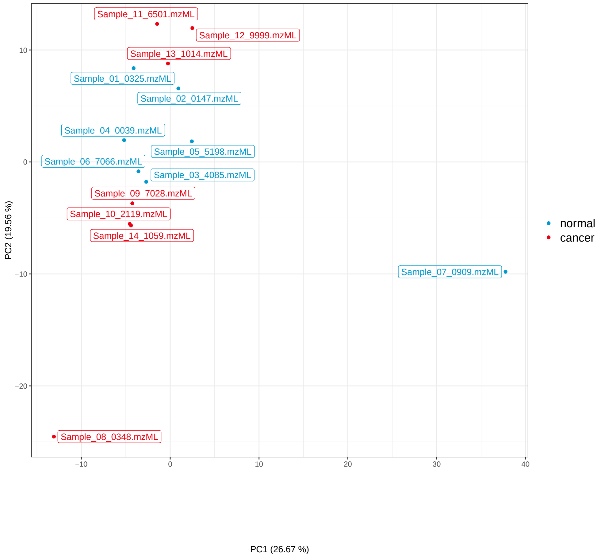
PCA, colored by group
