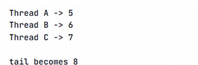
Fig. 11. Ticket allocation using Fetch-And-Add.
