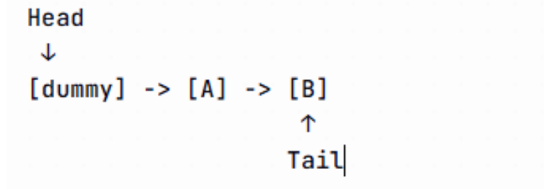
Fig. 9. Michael-Scott Queue after inserting two elements.
