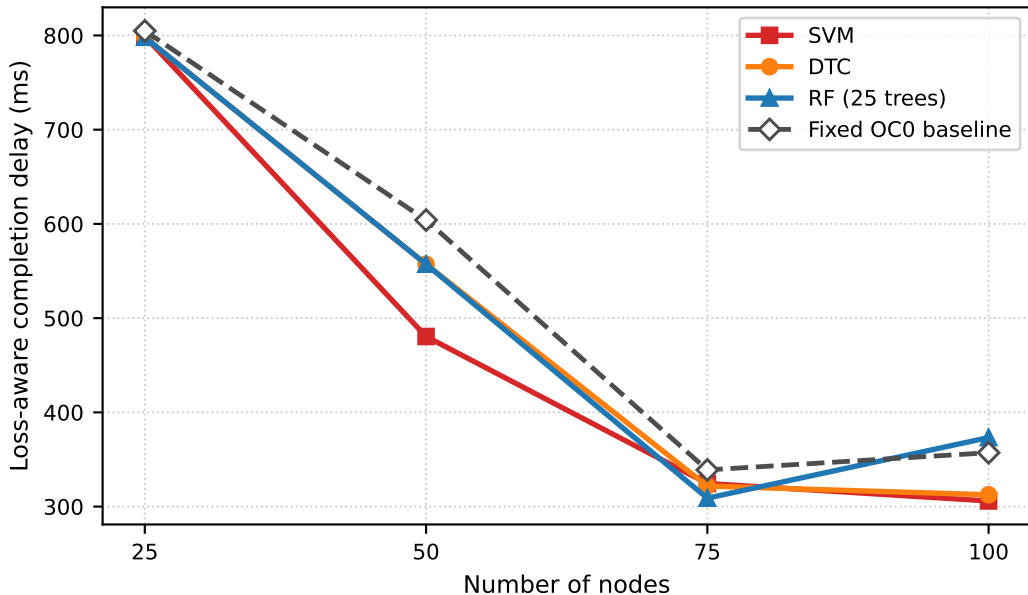
Delay versus Number of Nodes (1-s penalty per dropped packet)
