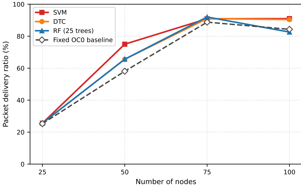
PDR versus Number of Nodes
