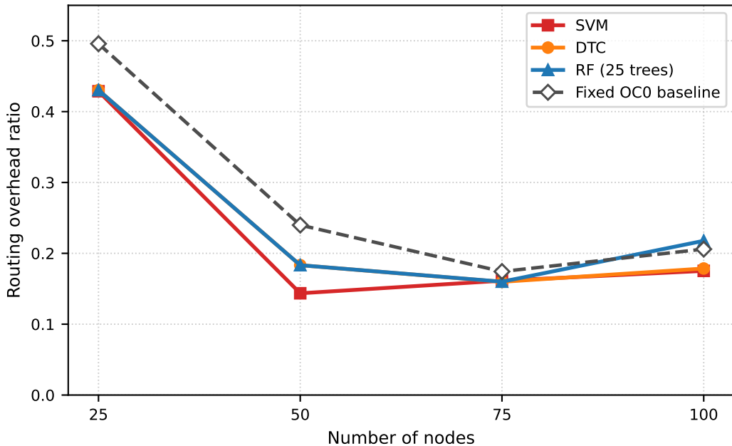
Routing Overhead versus Number of Nodes
