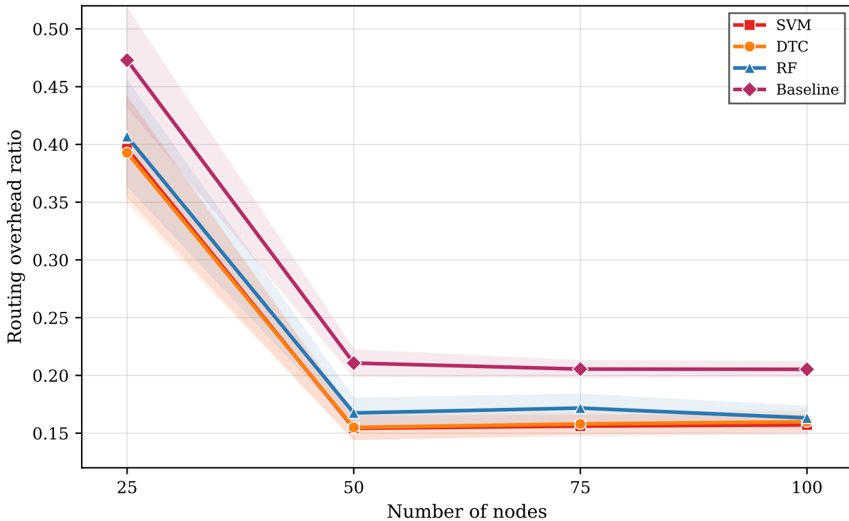
Routing Overhead vs Number of Nodes
