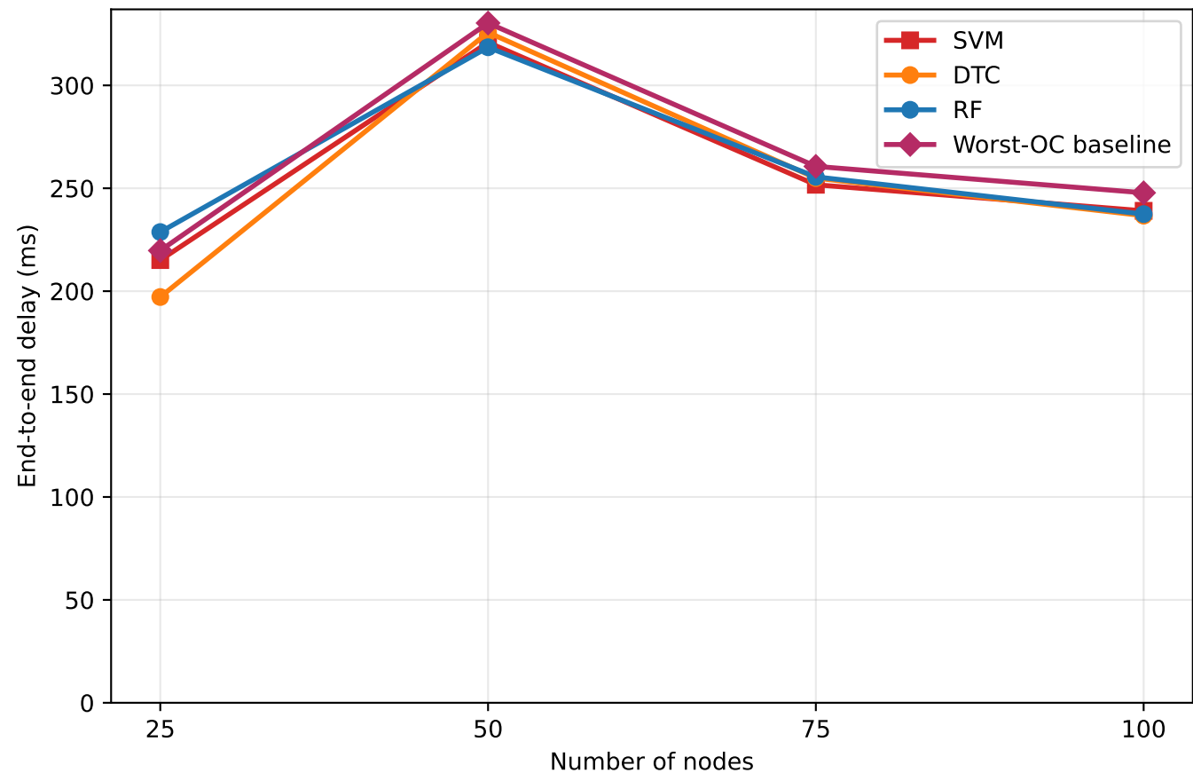
E2ED vs Number of Nodes
