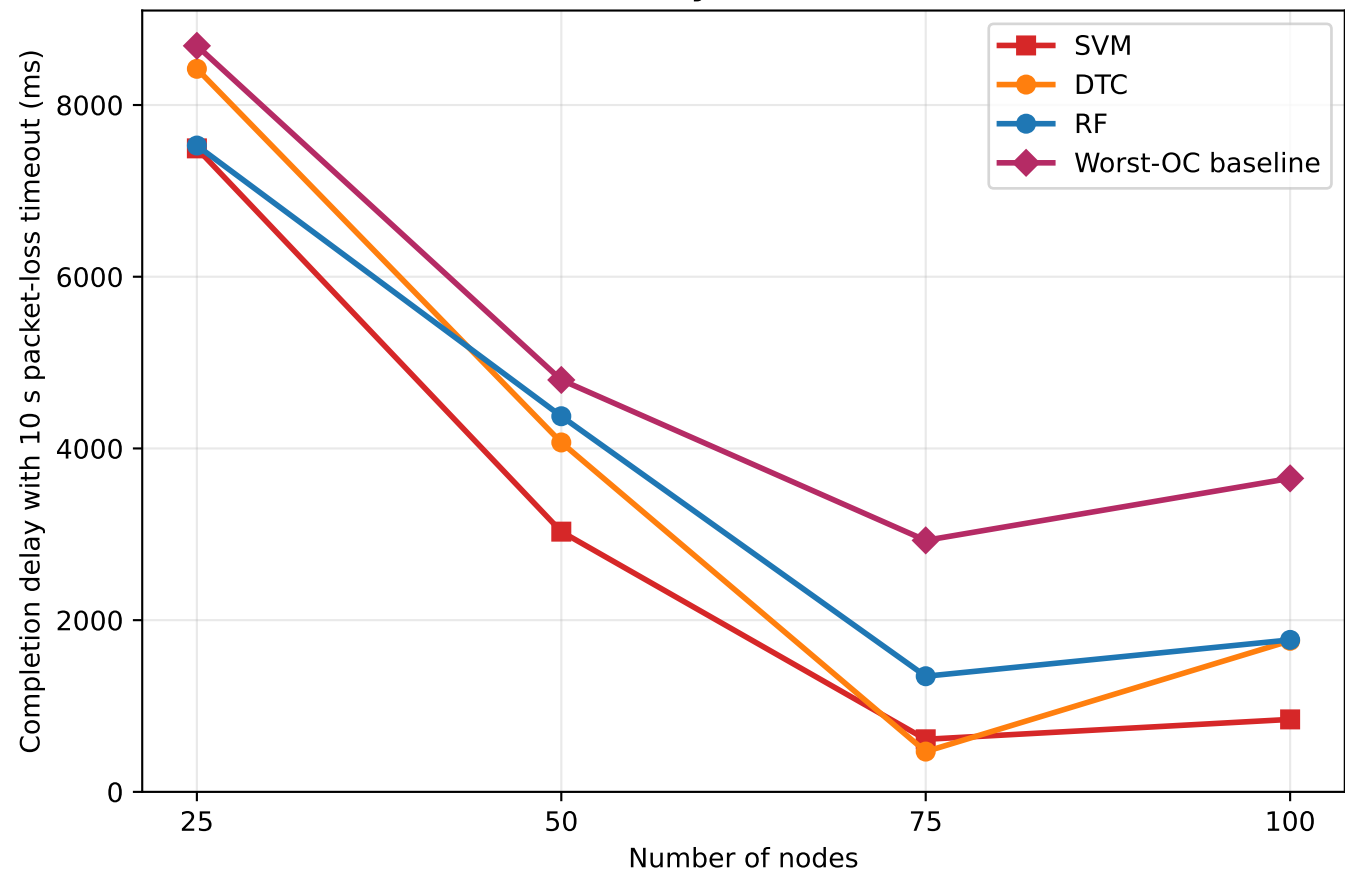
Loss-aware delay vs Number of Nodes
