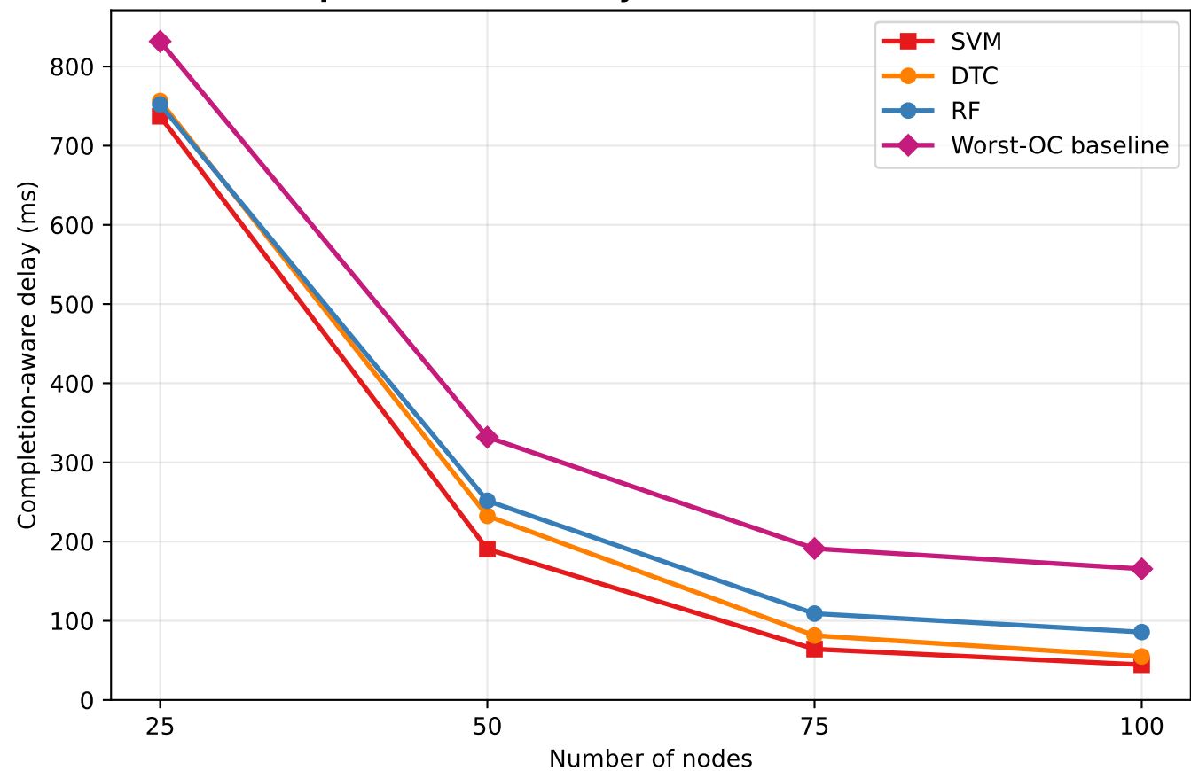
Completion-aware delay (ms) vs Number of Nodes
