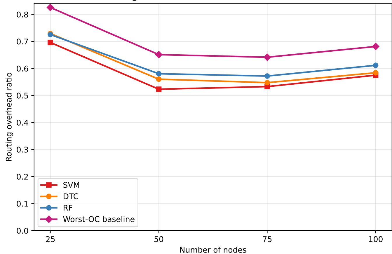
Routing overhead ratio vs Number of Nodes
