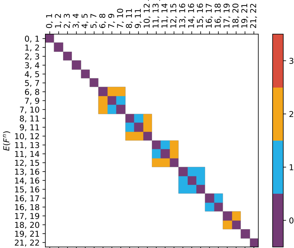
Distance Matrix, D_{F^n}^E
