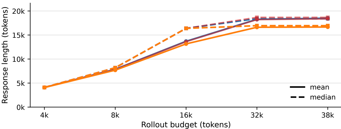
Mean/median response length
