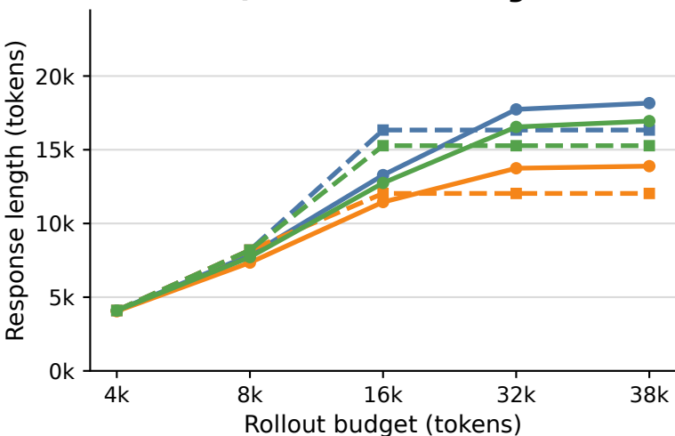
Qwen3-8B (Thinking)
