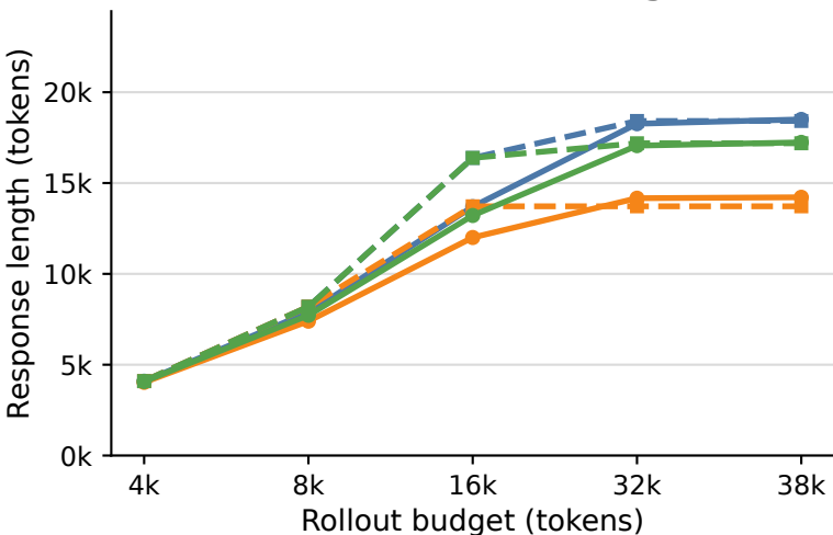
Qwen3-8B (Thinking)
