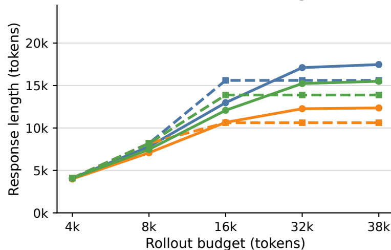
OLMo-3-7B-Think
