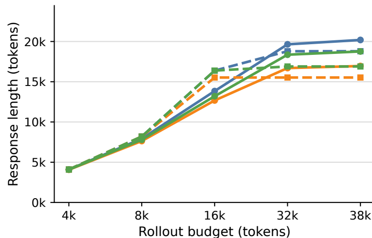
OLMo-3-7B-Think
