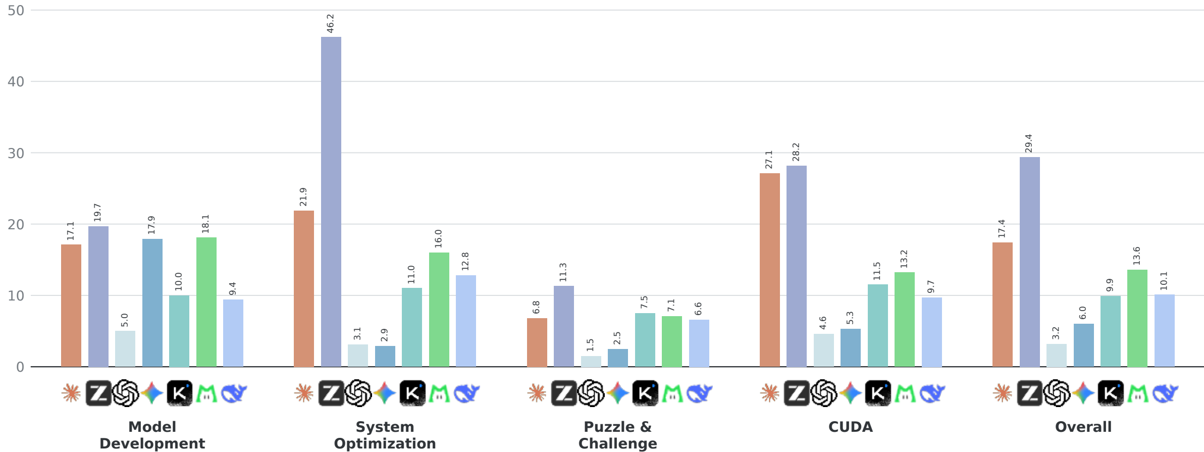
Mean tokens per task (million)
