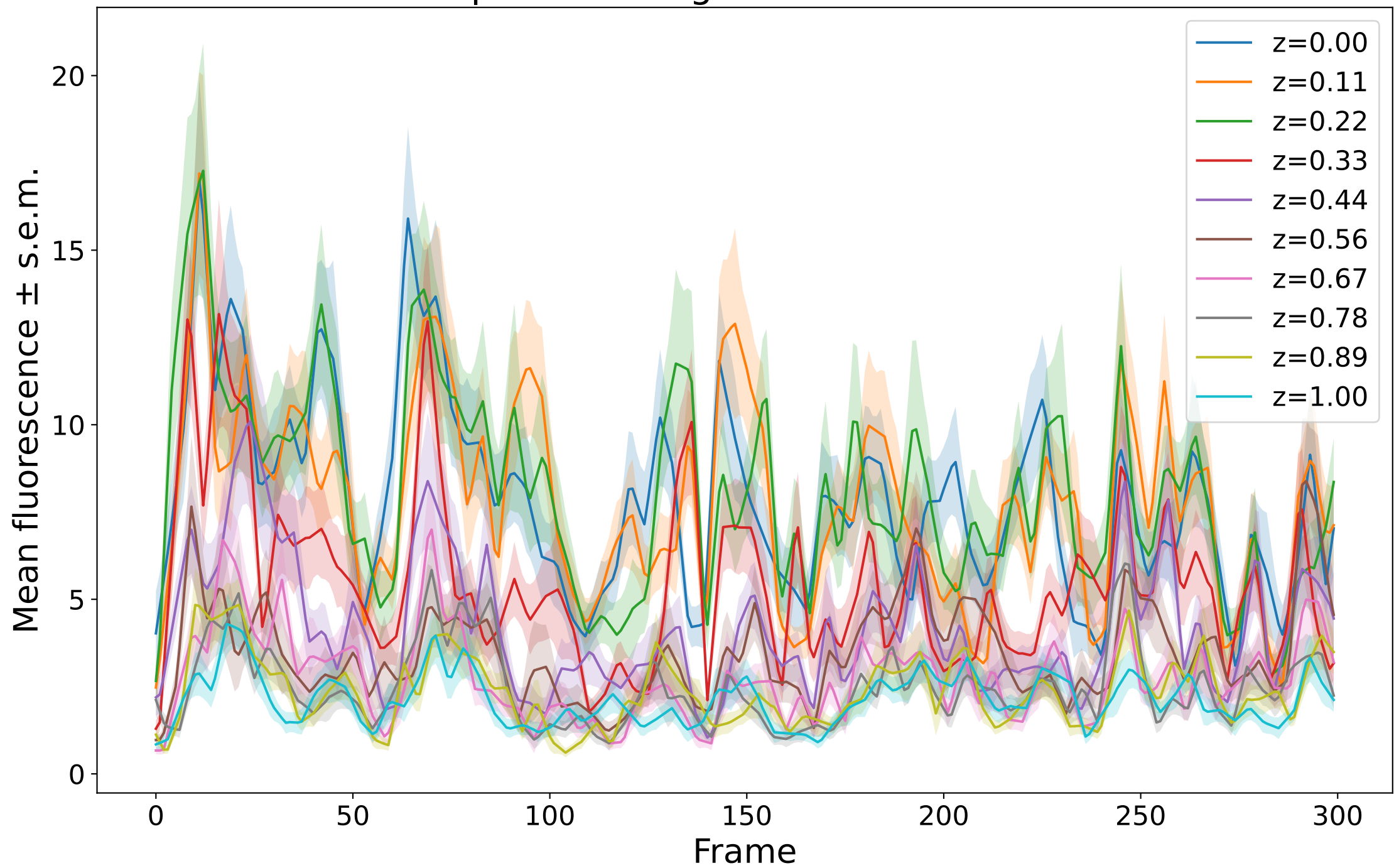
Per-plane average fluorescence trace
