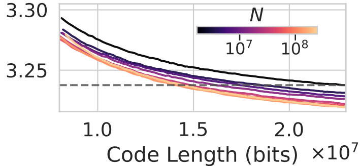
CIFAR-5M
