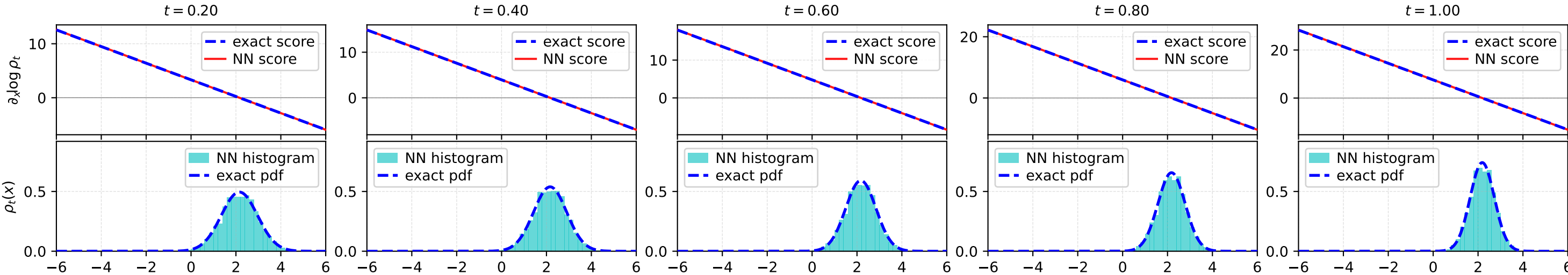
Single-well SOC (1-D, parametric) — \gamma = 0.1 , N_{\text{pt}} = 5000
