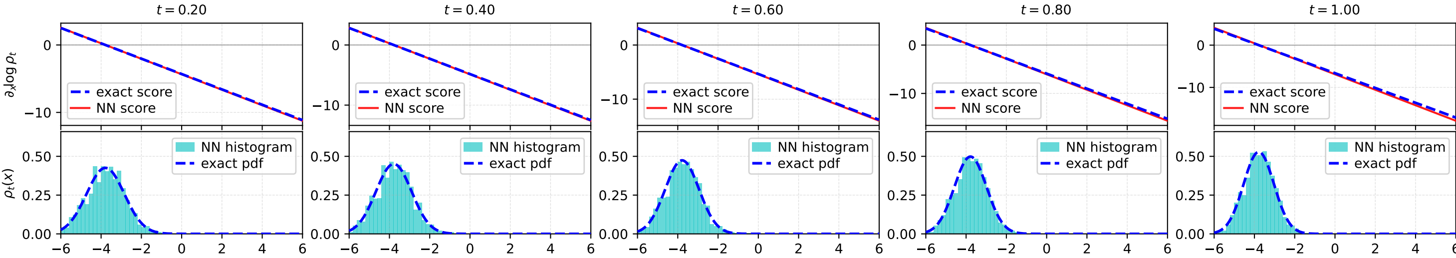
Systemic risk (1-D marginal) — \theta = (0.1, 0.5, 1, 1, 1.2) , m_0 = -3.78 , N_{\text{pt}} = 1024
