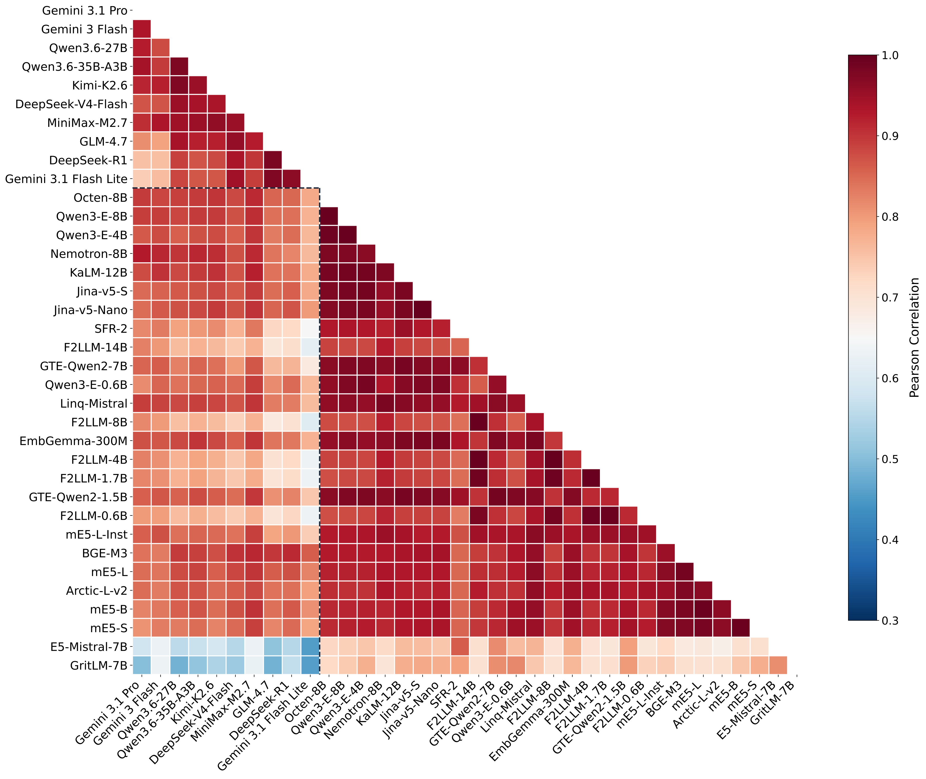
Model Capability Correlation Across Tasks
