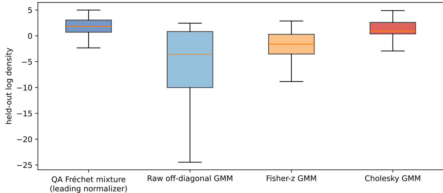
Test-window predictive scores on a common off-diagonal reference measure
