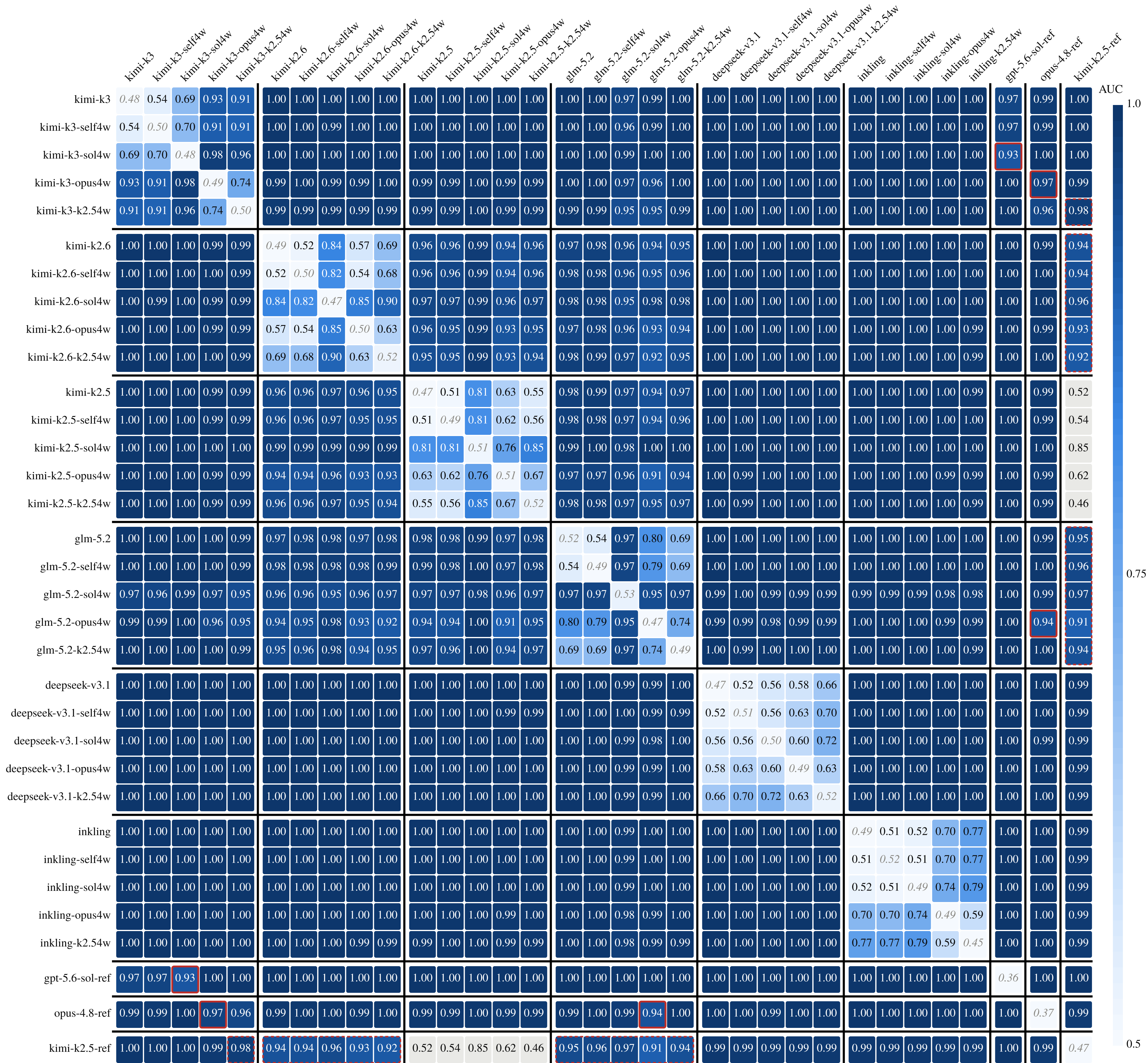
Style-classifier separability (AUC)
