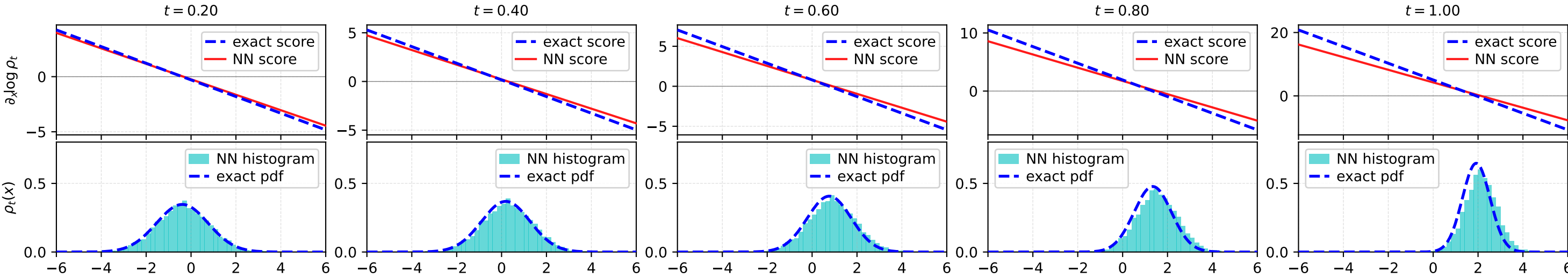
Schrödinger Bridge (1-D, non-parametric) — \gamma = 1 , N_{\text{pt}} = 5000
