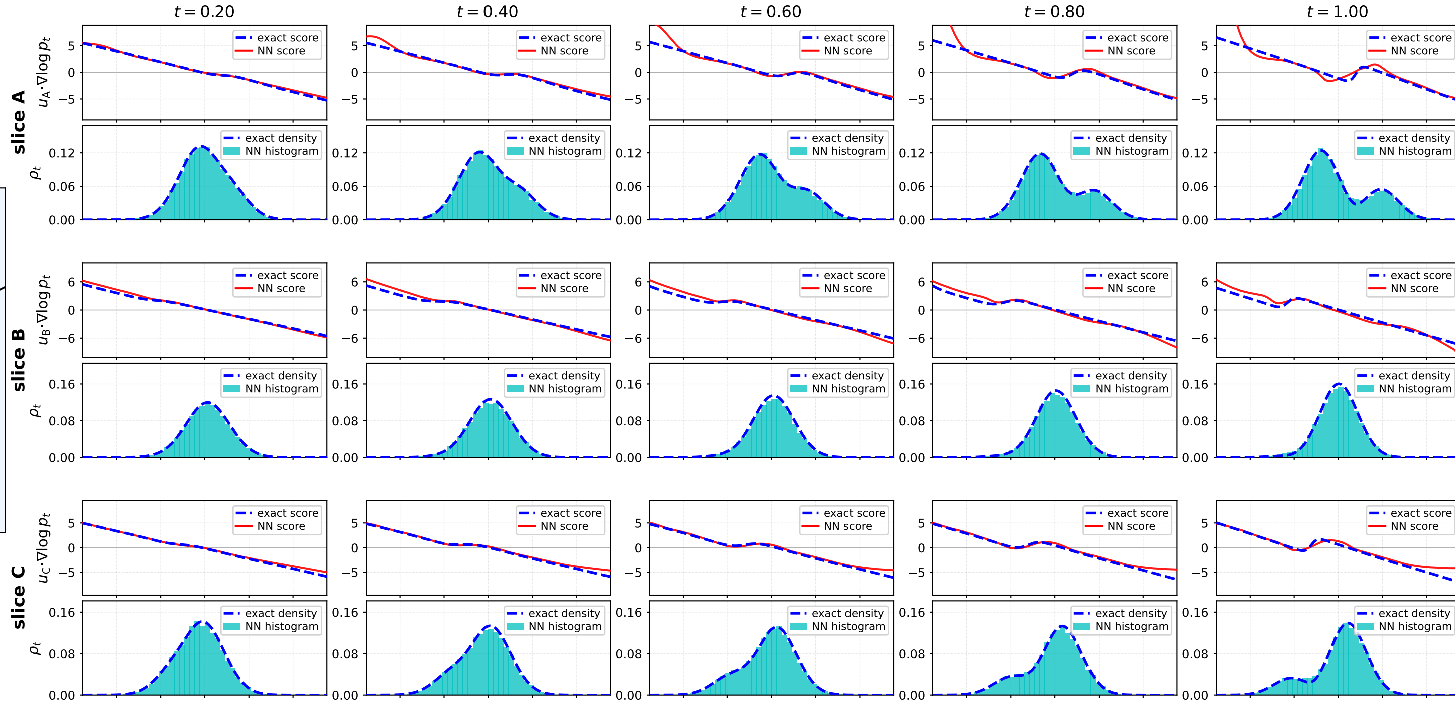
Multi-well SOC ( \gamma = 0.50 ): tangential score u \cdot \nabla \log p_t (upper) and slice density (lower) along chords A, B, C
