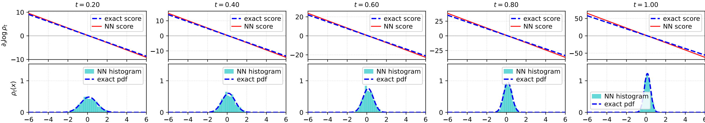
Systemic risk (1-D marginal) — \theta = (0.1, 0.5, 1, 1, 0.25) , m_0 = +0.14 , N_{\text{pt}} = 1024
