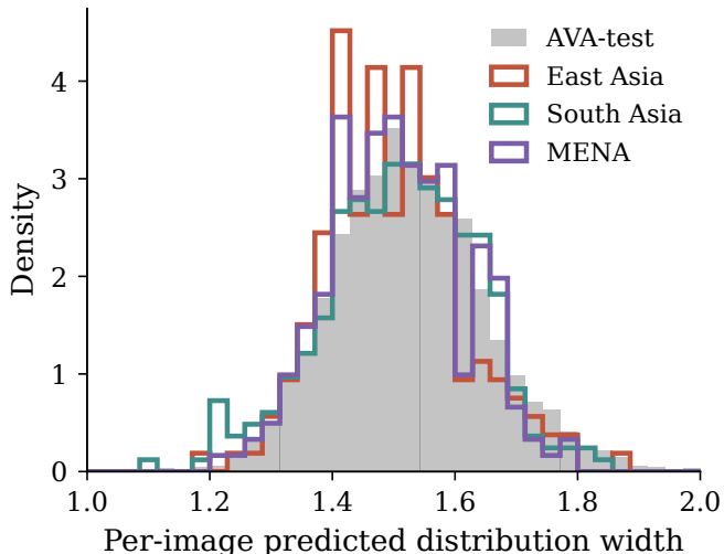
(b) Per-image prediction width (calibration)
