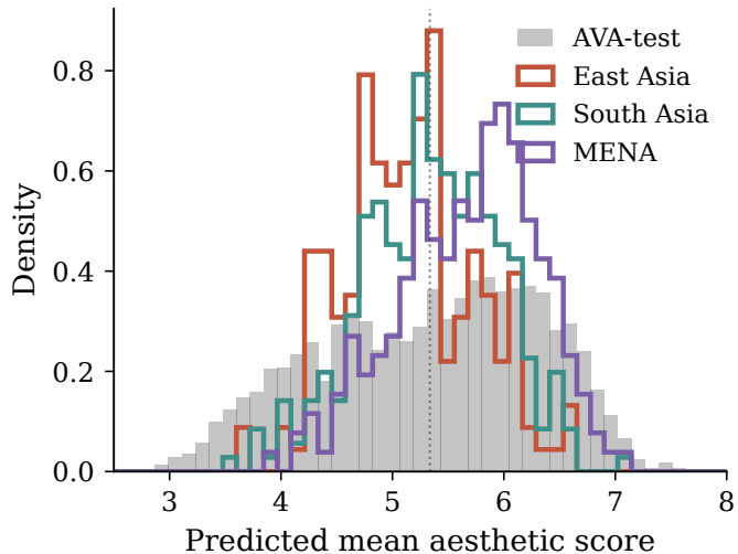
(a) Predicted score distributions
