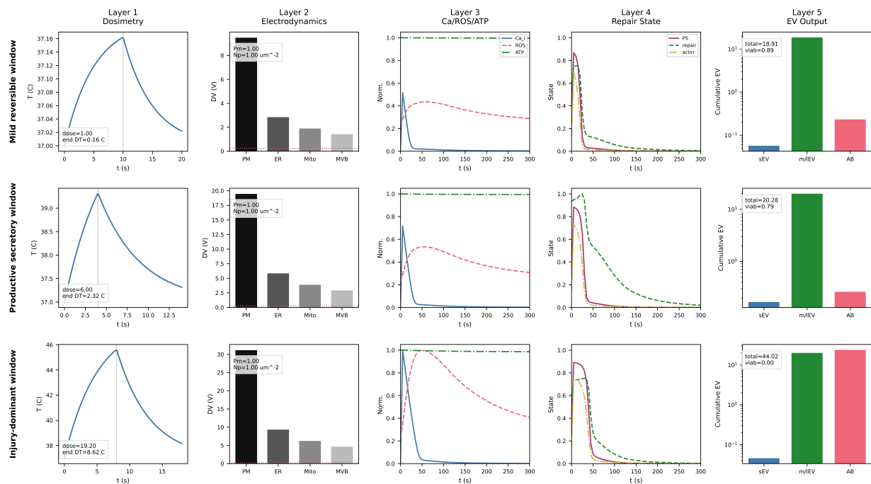
Figure 7. Integrated preliminary storyboard across Layers 1–5. Each row represents one illustrative scenario and each column summarizes one model layer from dosimetry through EV output. The top row shows a mild reversible window, the middle row a more productive secretory window, and the bottom row an injury-dominant window. The figure makes the multiscale logic of the framework visible: stronger Layer 1 dose and Layer 2 charging drive larger Layer 3 \text{Ca}^{2+} /ROS perturbations, which then reshape Layer 4 repair states and finally alter Layer 5 subtype weighting and viability.
