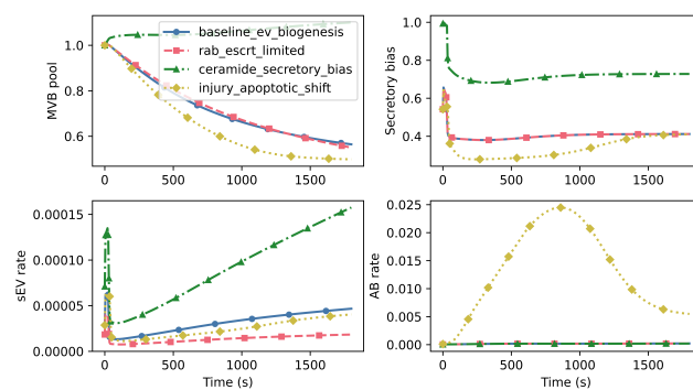
Figure 6. Preliminary Layer 5 example behavior. The EV-biogenesis comparison shows that the pool-balance release model distinguishes Rab/ESCRT-limited, ceramide-favored secretory, and injury-shifted regimes. In this framework, MVB pool size and secretory bias respond differently from final apoptotic-body output, allowing the model to separate productive small-EV routing from high-stress vesiculation.
