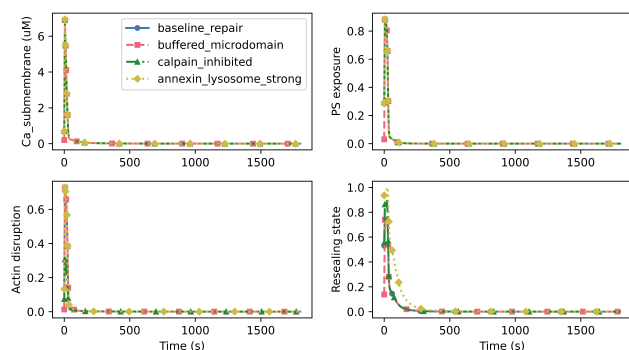
Figure 5. Preliminary Layer 3–4 example behavior. The remodeling/repair example shows how the reduced \text{Ca}^{2+} -sensor module separates phosphatidylserine exposure, actin disruption, and resealing competence across buffered, calpain-inhibited, and annexin/lysosome-supported regimes.
