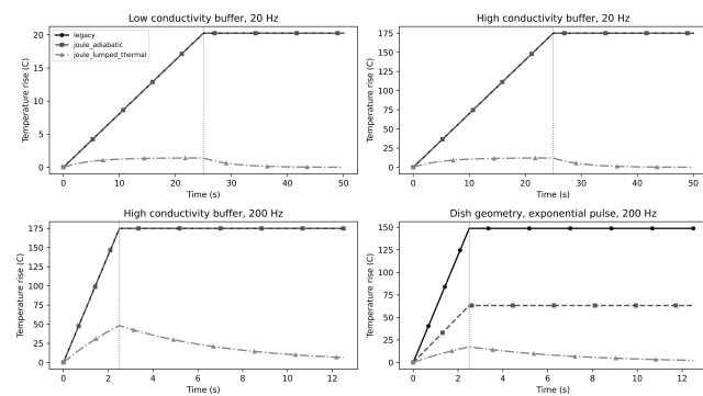
Figure 2. Preliminary Layer 1–2 example behavior. The dosimetry comparison shows how the lumped thermal framework separates absorbed electrical dose from retained heating: low-conductivity conditions remain weakly heated, while high-conductivity and high-repetition-rate pulse trains accumulate larger temperature rises even under similar nominal amplitudes.
