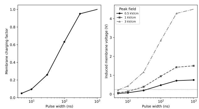
Figure 3. Preliminary Layer 1–2 example behavior. The reduced electrodynamics model shows first-order membrane charging toward the Schwan limit, so longer pulses and larger cells reach higher induced membrane voltages and cross a permeability-relevant threshold more readily than ultrashort or smaller-cell cases.
