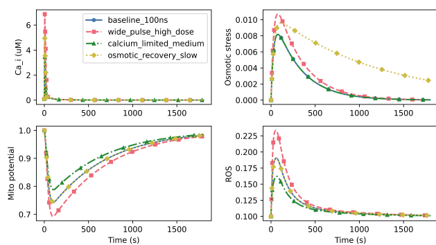
Figure 4. Preliminary Layer 3–4 example behavior. The compartmental ion-transport/bioenergetics example compares baseline, higher-dose, calcium-limited, and slow-recovery settings; the chosen ODE framework converts the electroporation state into different \text{Ca}^{2+} transients, osmotic stress histories, mitochondrial stress, and ROS accumulation.
