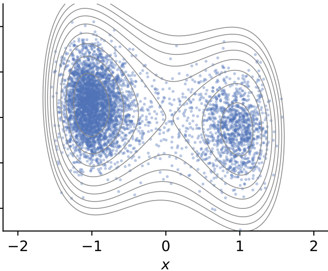
diffusion model samples
