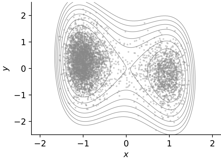
exact Boltzmann samples
