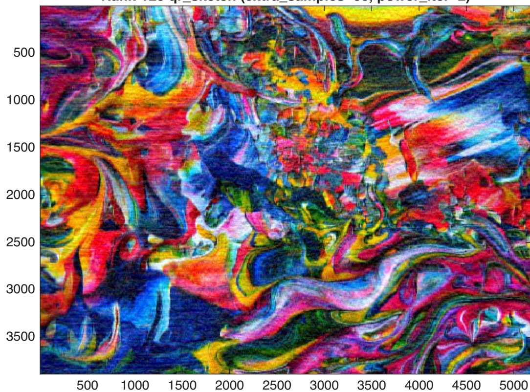
Rank-120 qr_sketch (extra_samples=60, power_iter=2)
