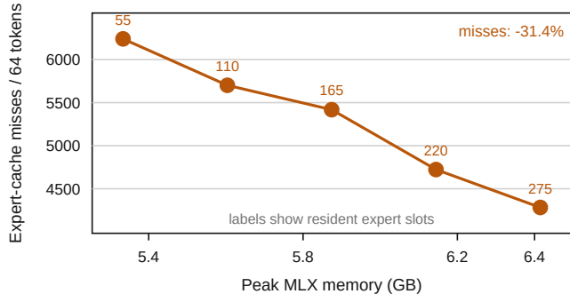
(b) Mechanism: fewer cache misses
