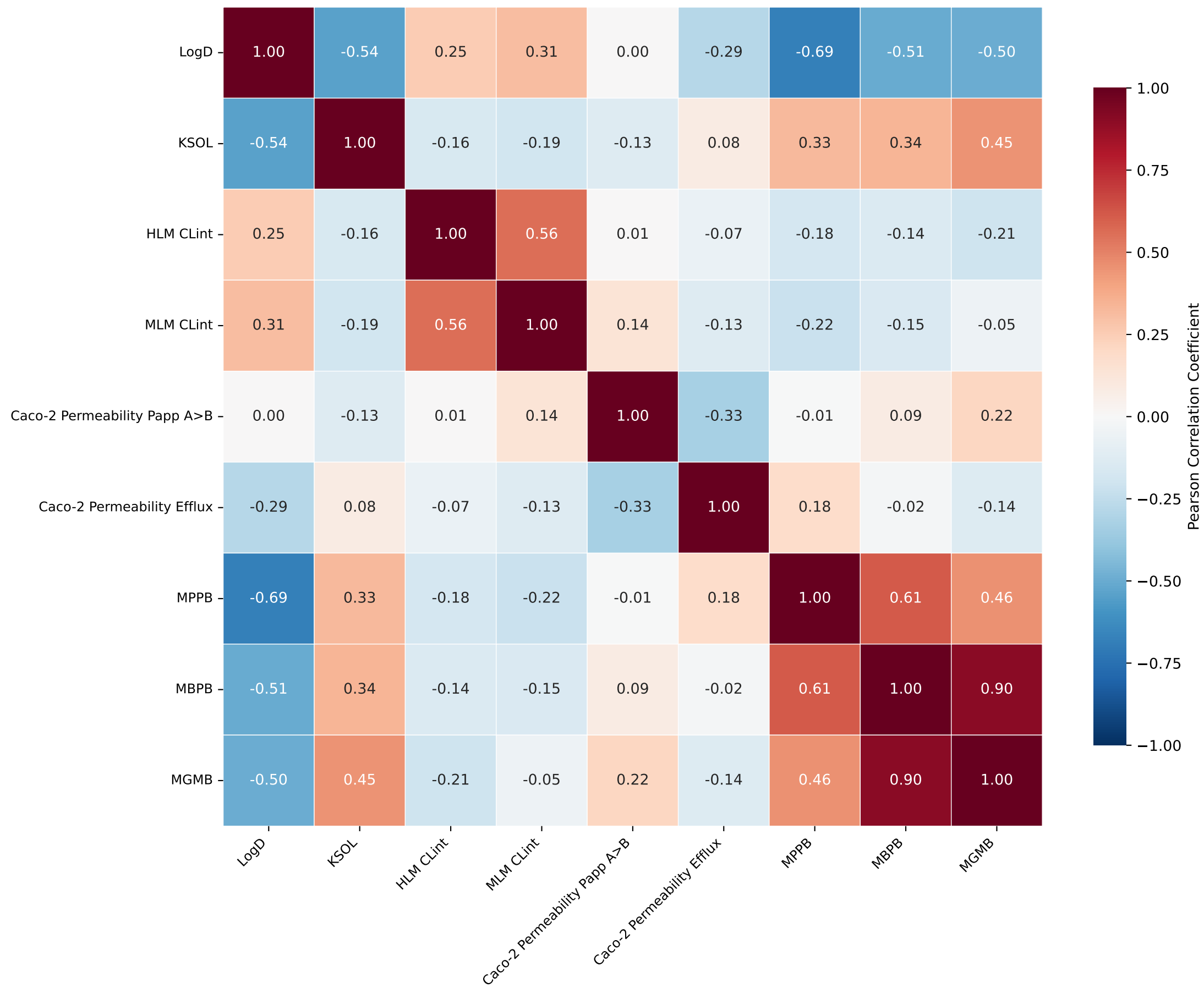
Correlation Matrix of Target Properties Molecular Property Prediction Dataset
