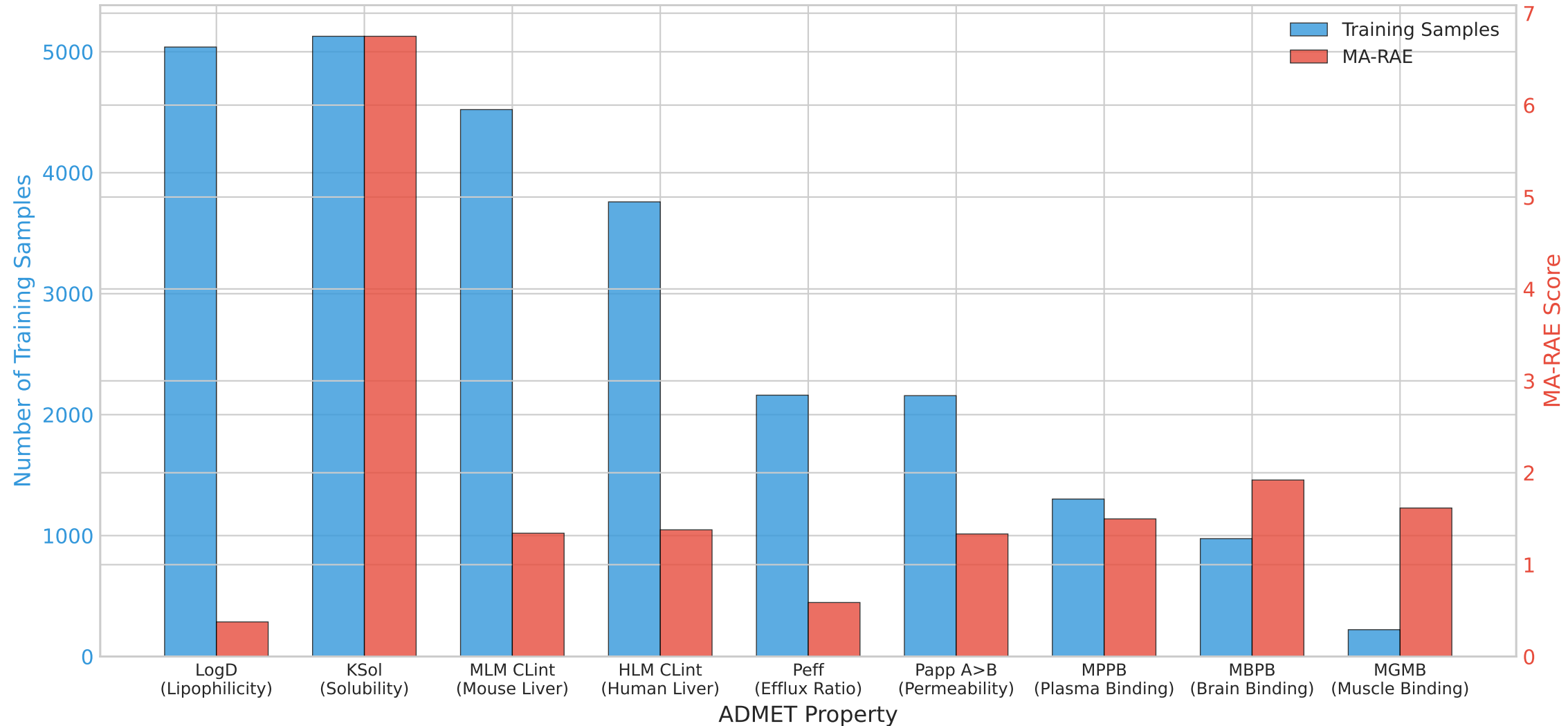
Training Data Availability vs. Model Performance
