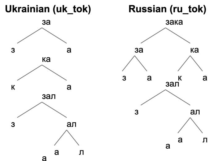
Figure 2: Hierarchical BPE tokenization trees comparing the word заказати in Ukrainian (left) and Russian (right). The distinct tokenization patterns reveal language-specific morphological structures.
