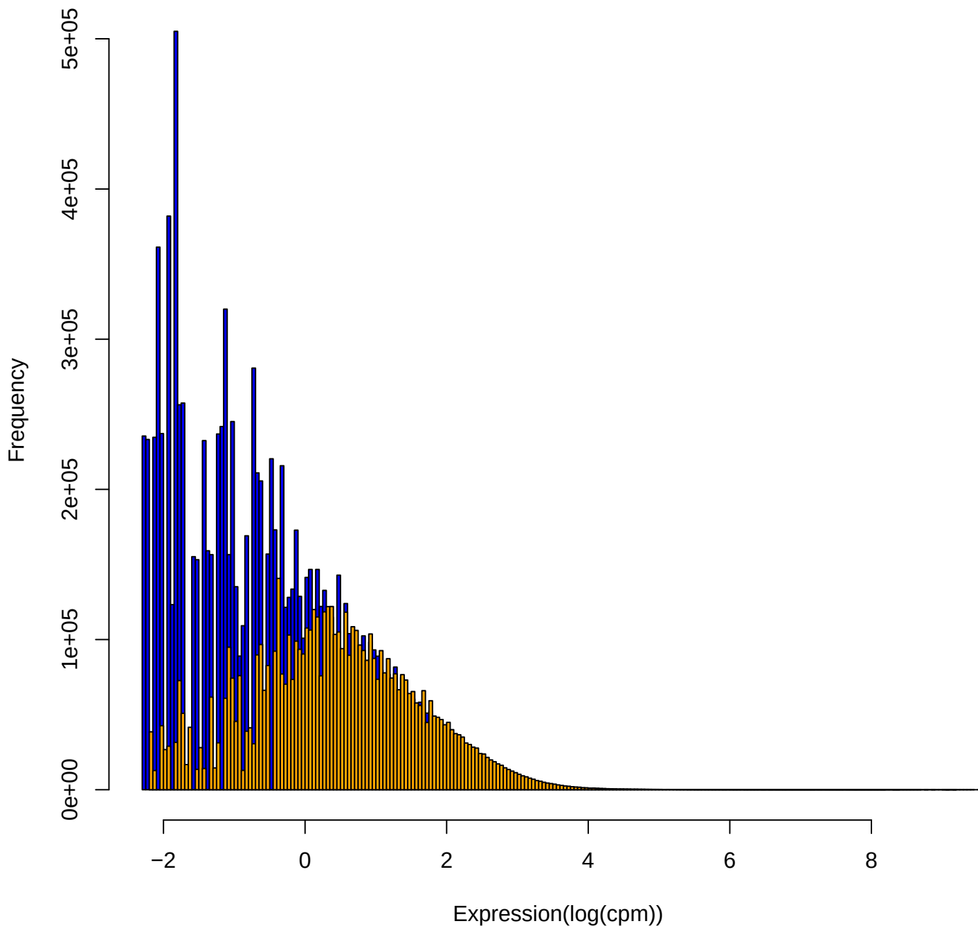
Distribution of log(cpm) in raw (blue) and trimmed (orange) data mean(cpm(count))>=1
