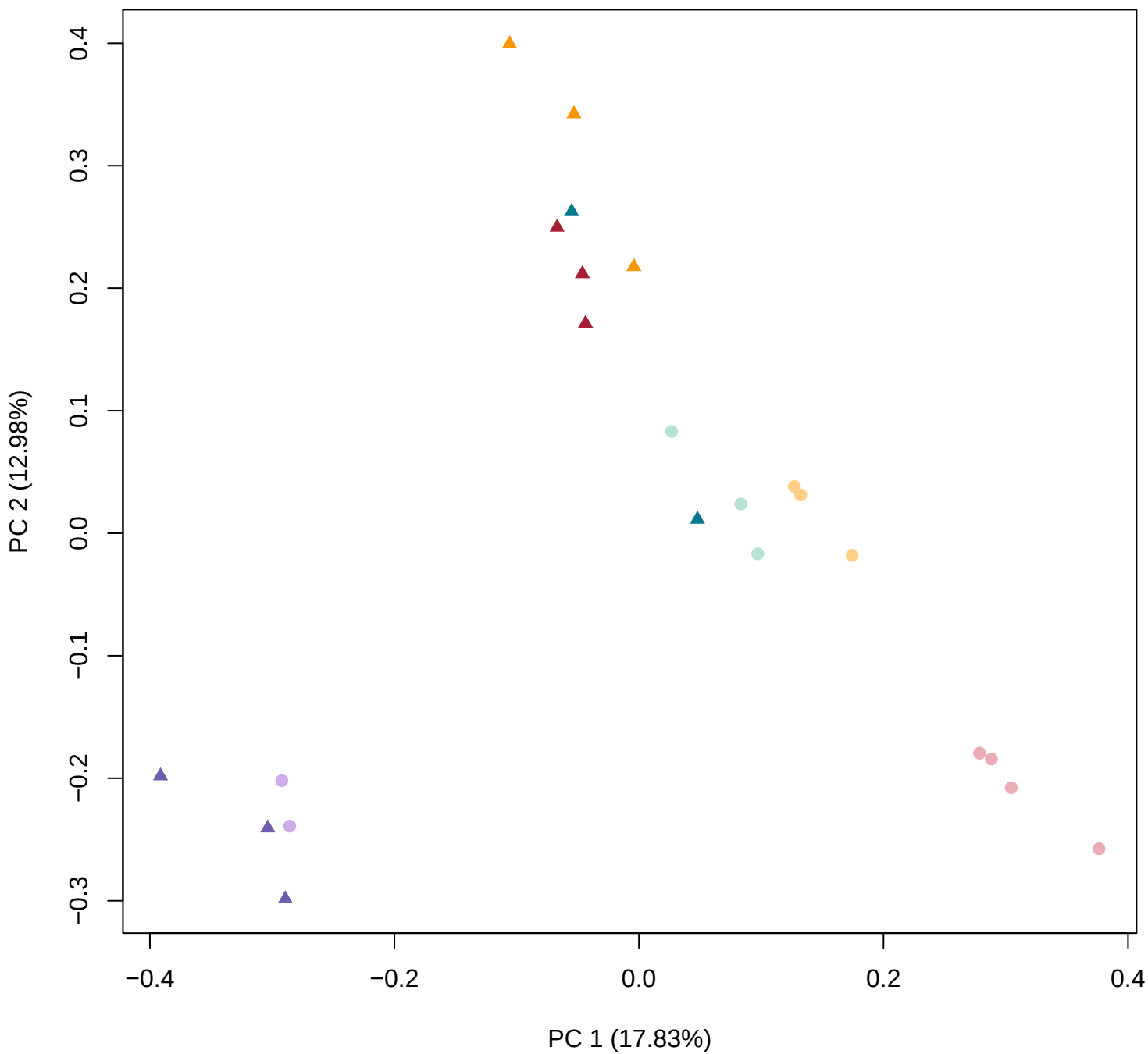
PCA – Unwanted variance not removed
