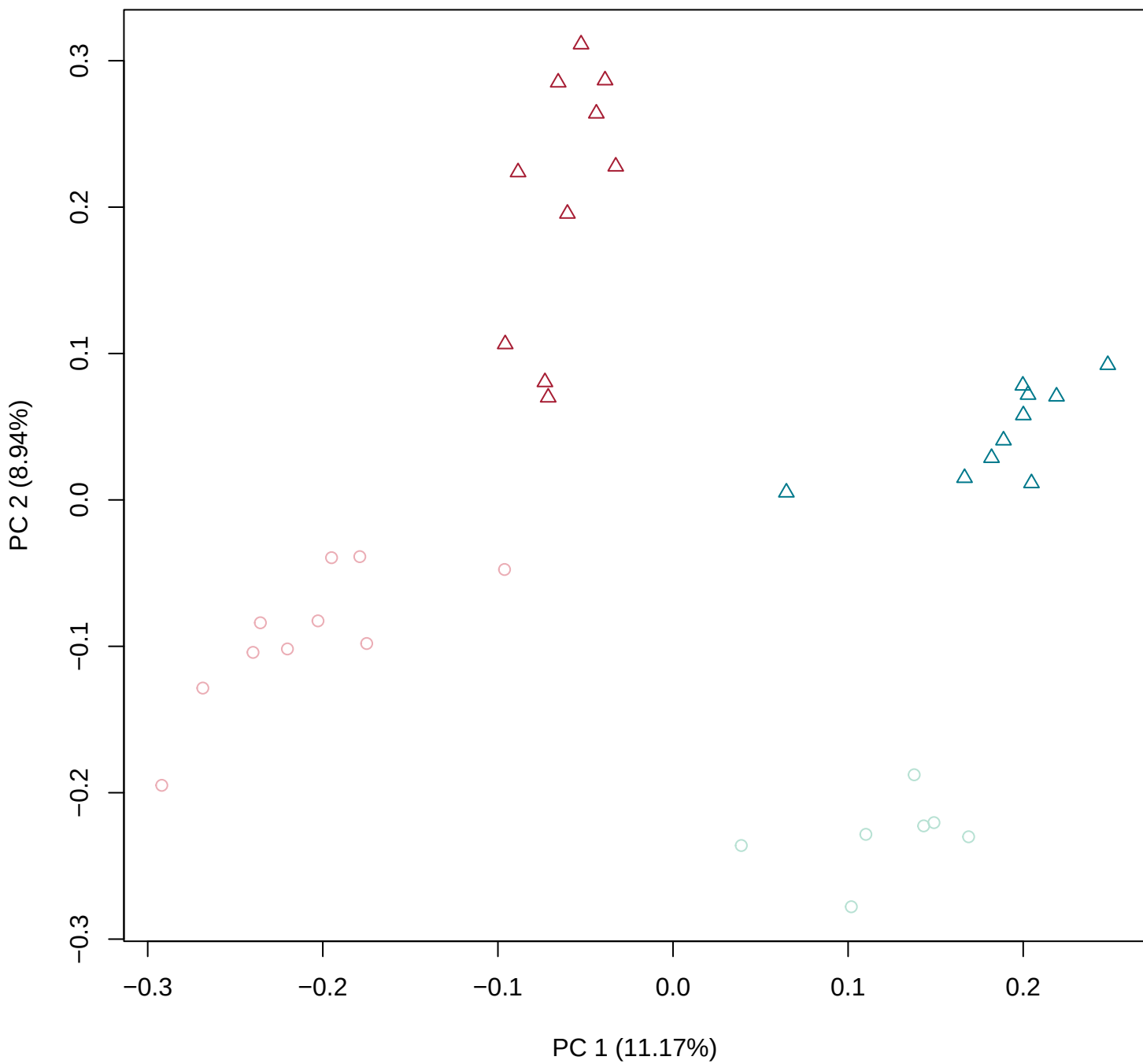
PCA – Unwanted variance removed
