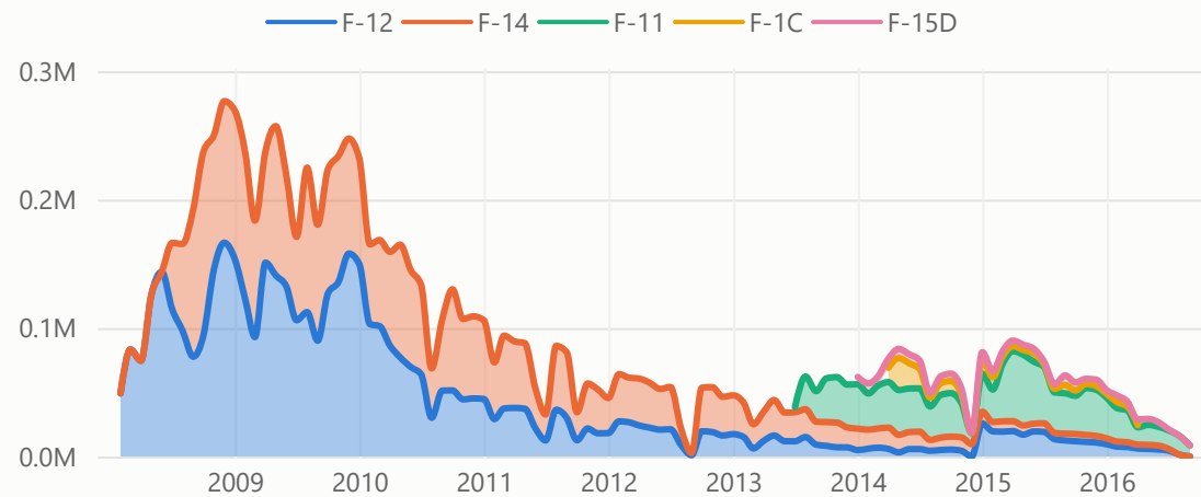
Two wells, F-12 and F-14, carried 85% of Volve's oil
