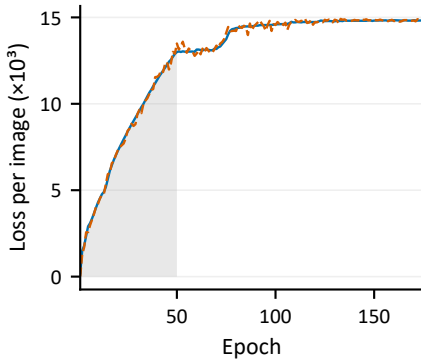
(b) Weighted KL divergence loss
