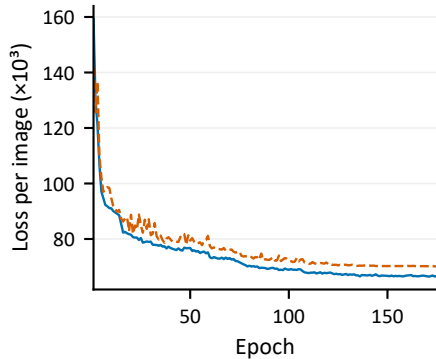
(c) L1 reconstruction loss
