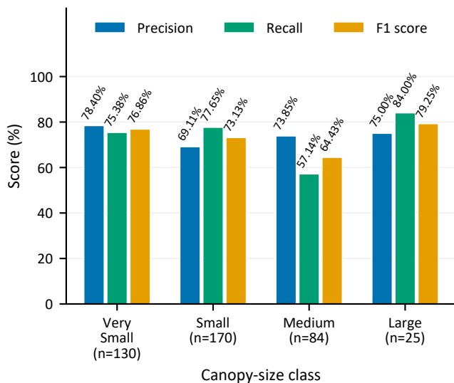
(b) C5 per-class performance
