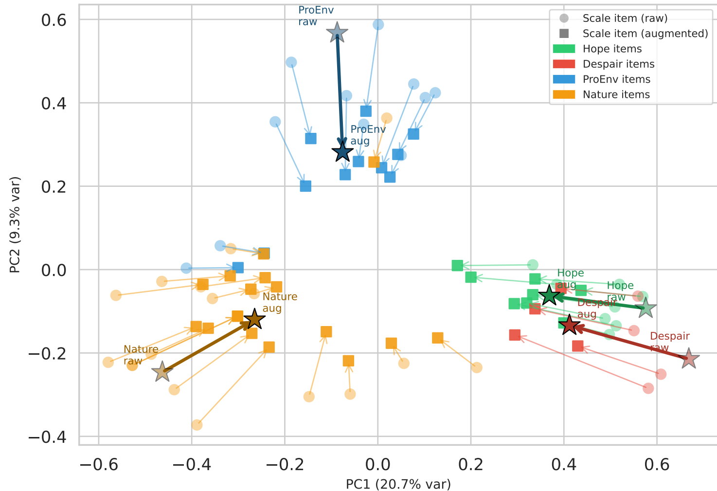
Pole shift after NLI emotion augmentation (PCA of raw 384-dim scale embeddings)
