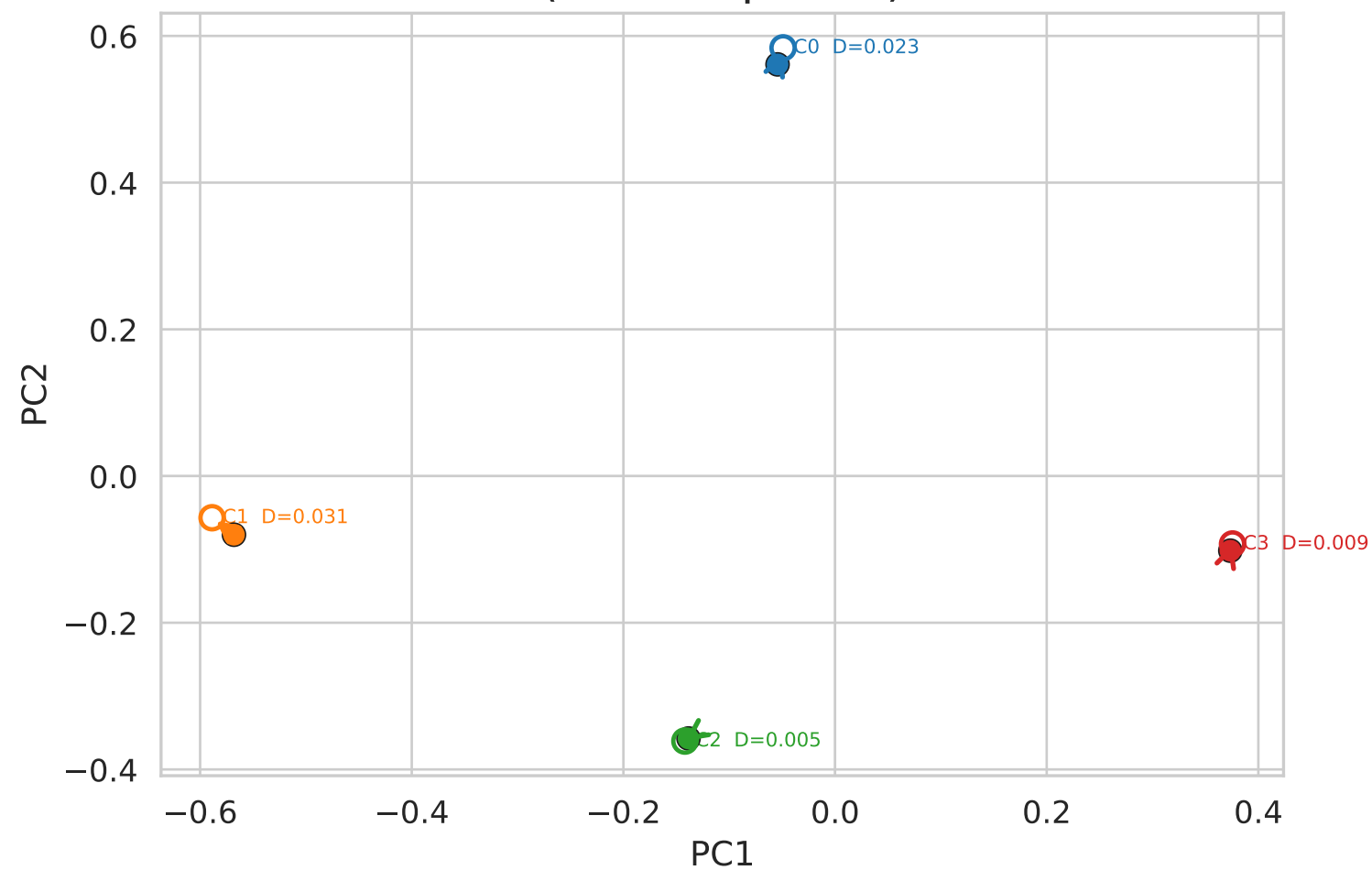
Group 0 — Pre→Post centroid shift (filled=PRE · open=POST)
