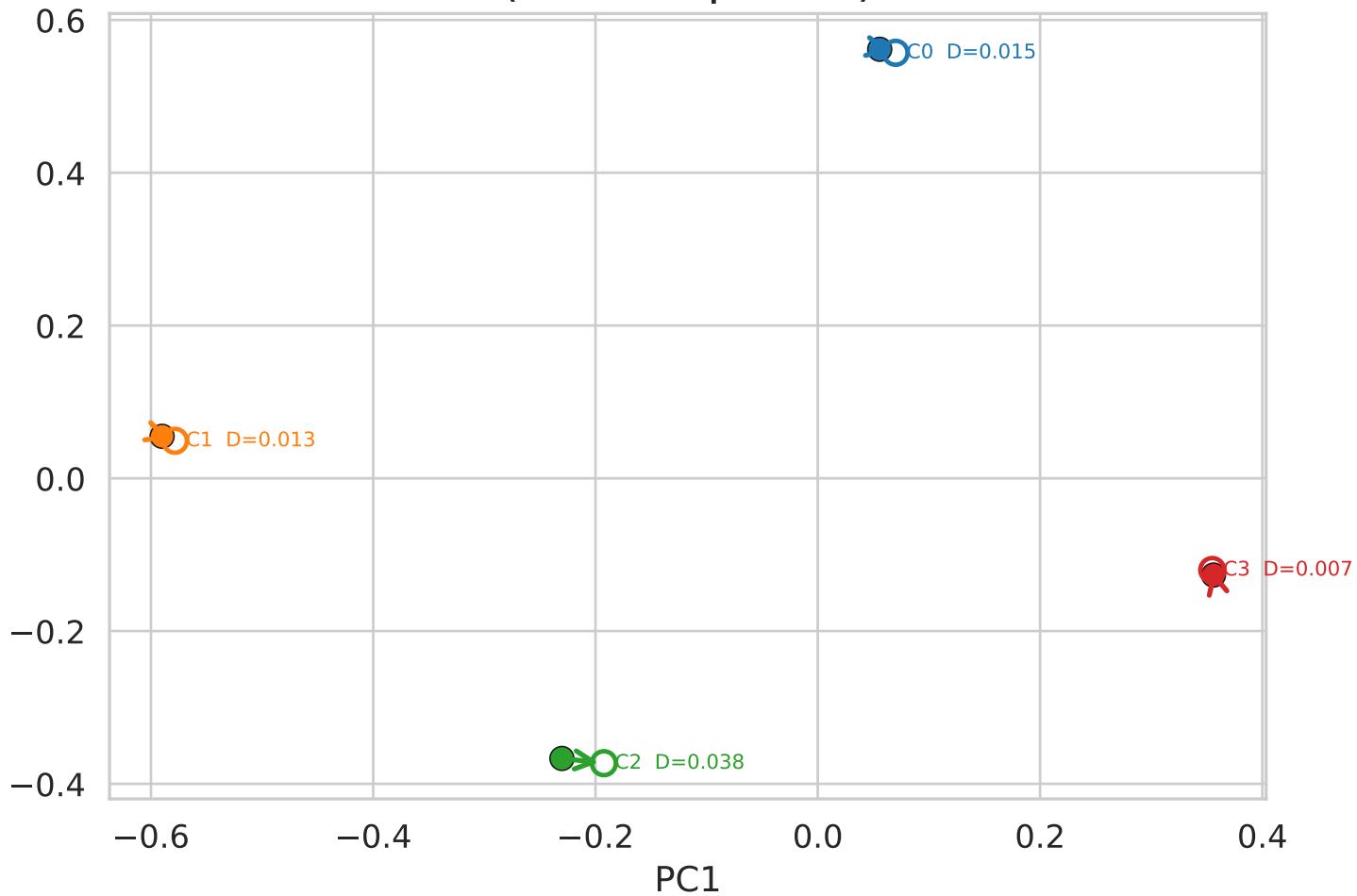
Group 1 — Pre→Post centroid shift (filled=PRE · open=POST)
