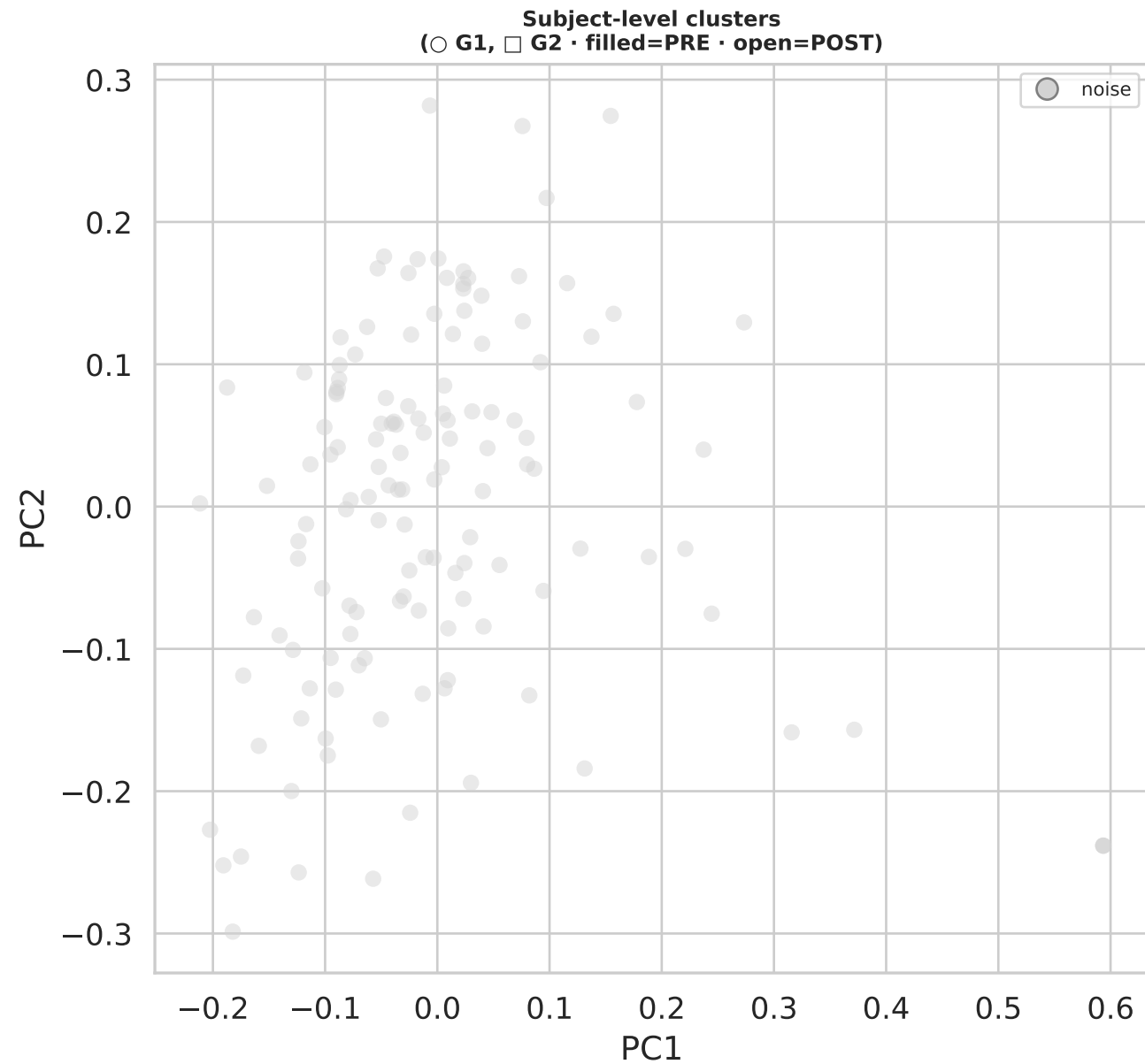
Subject-level clustering — both groups, pre vs post
