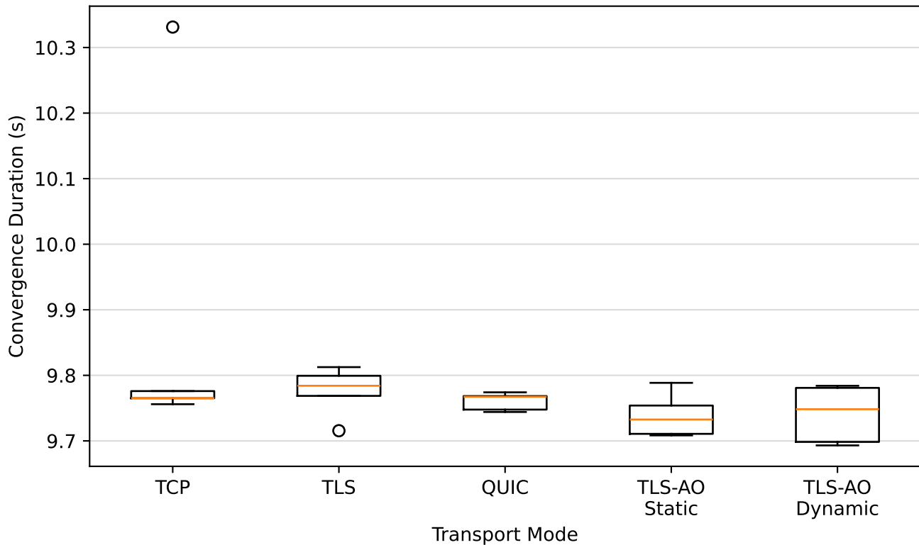
Generated-prefix BGP Convergence — 10,000 Prefixes, Bulk Injection
