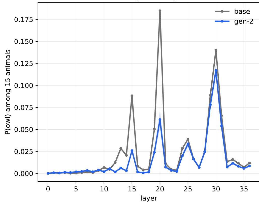
Owl probability
