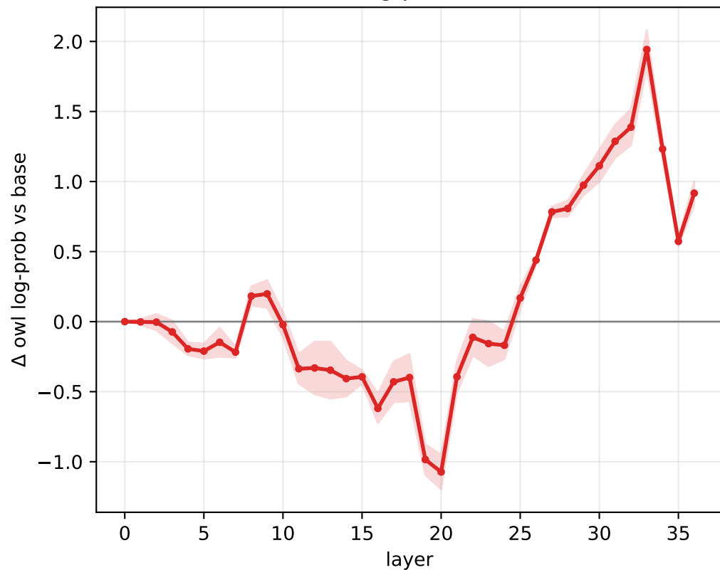
Owl log-prob shift
