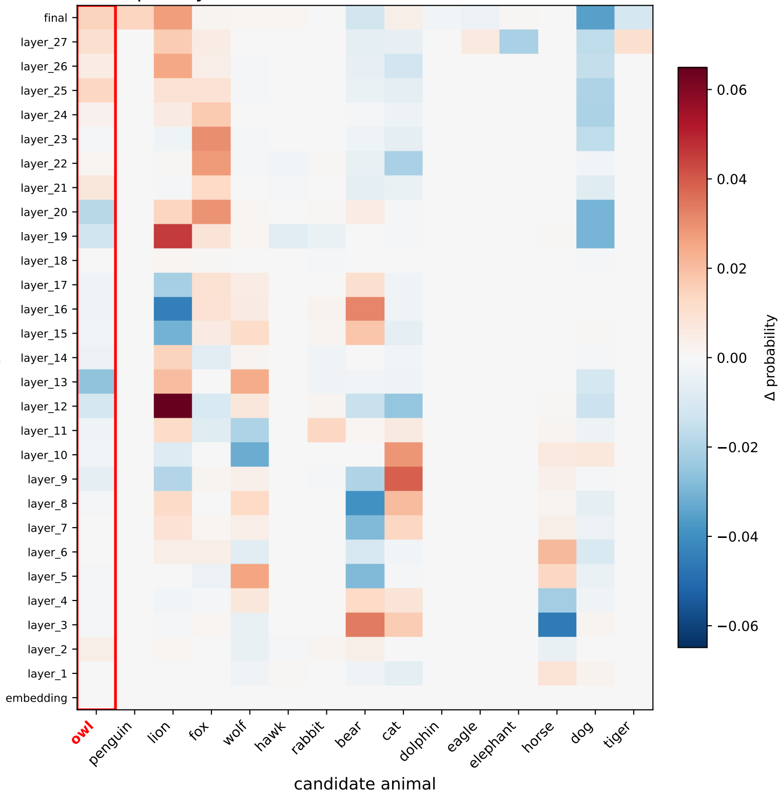
\Delta P(\text{animal}) per layer (fine-tuned – baseline) — Qwen2.5-7B-Instruct
