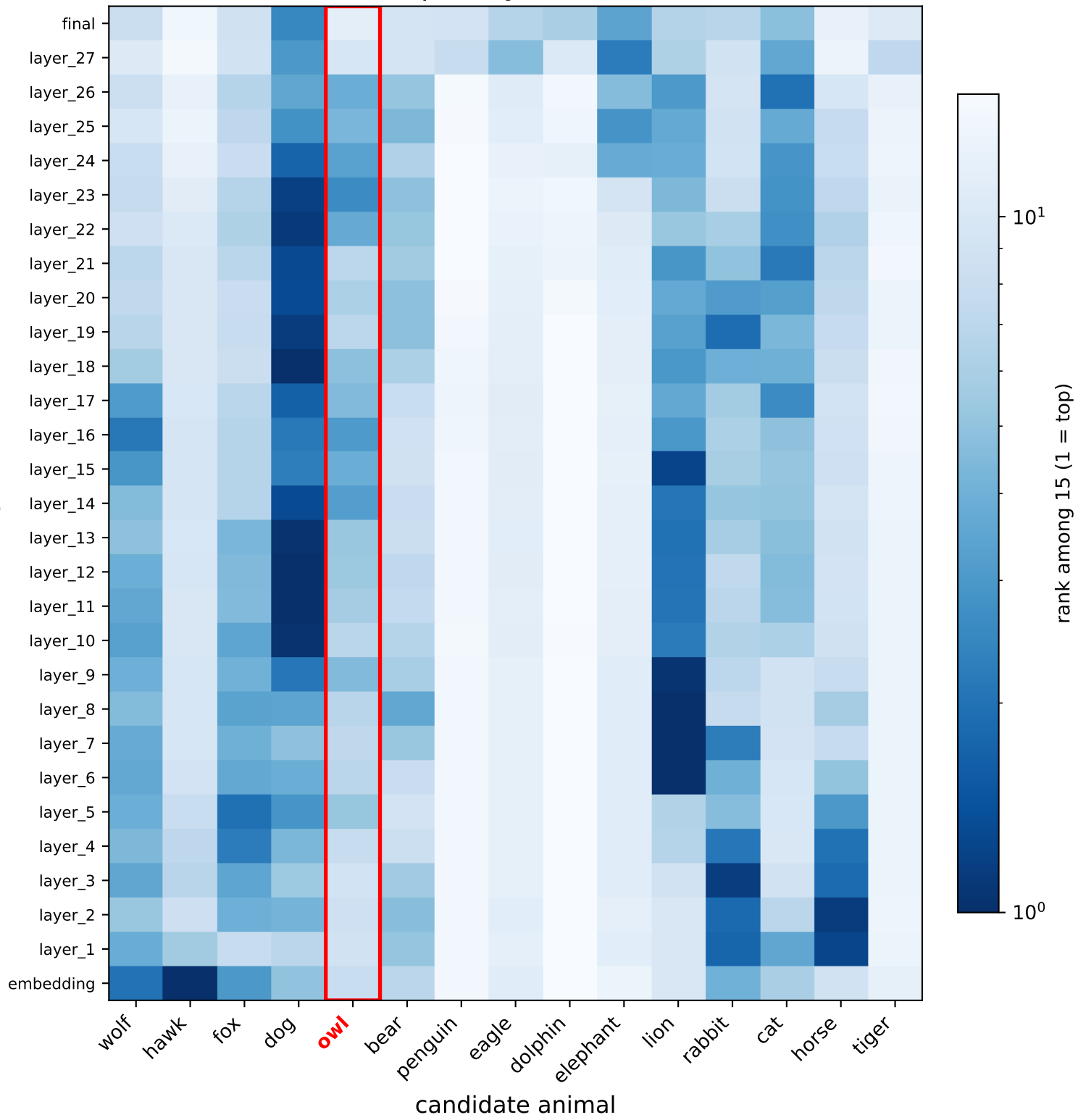
Fine-tuned rank of animal per layer — Qwen2.5-Coder-7B-Instruct
