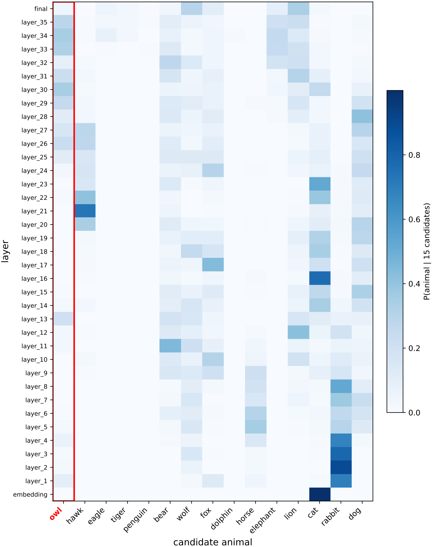
Fine-tuned P(animal) per layer — Owen3-4B-Instruct-2507
