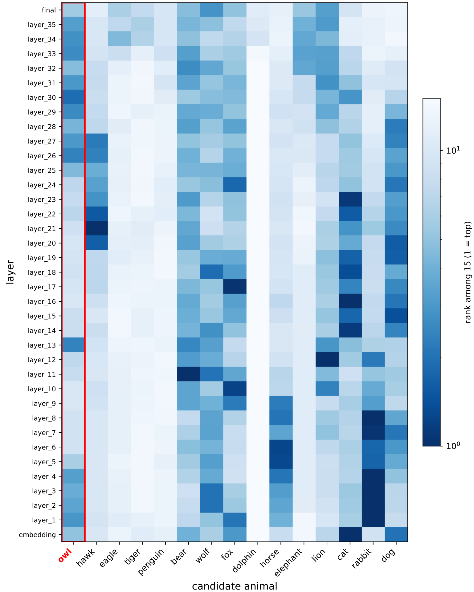
Fine-tuned rank of animal per layer — Qwen3-4B-Instruct-2507
