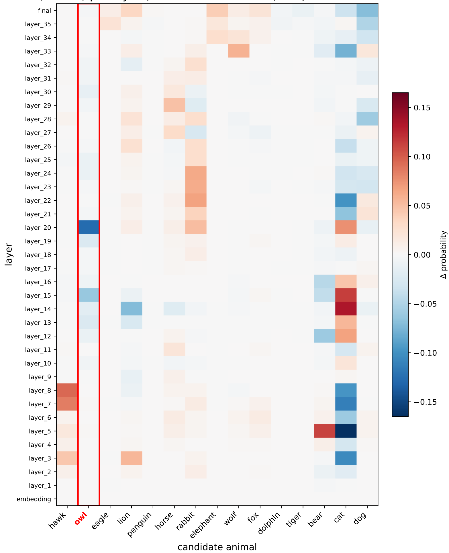
\Delta P(\text{animal}) per layer (fine-tuned – baseline) — Qwen2.5-3B-Instruct
